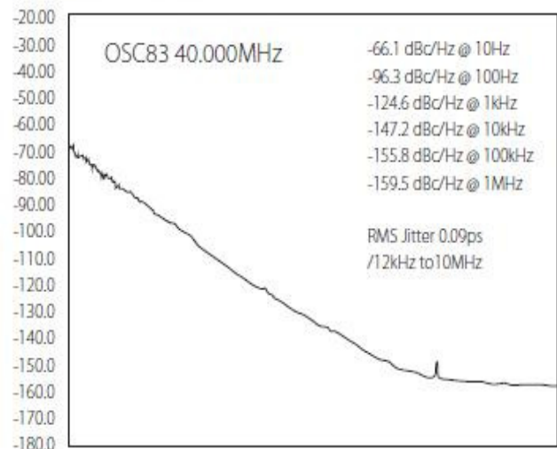
Phase Noise
