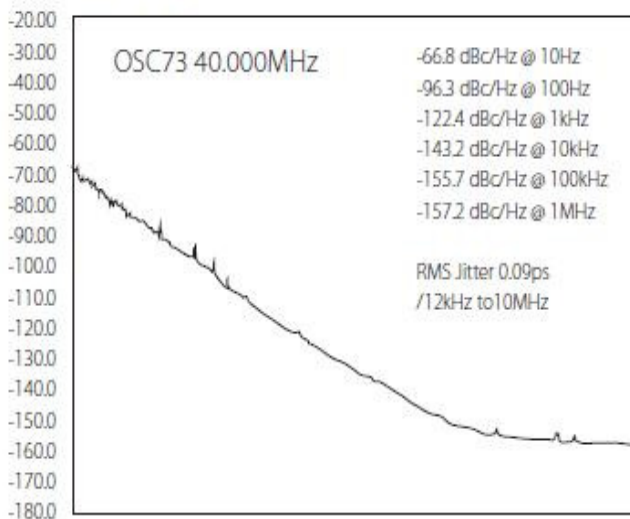
Phase Noise
