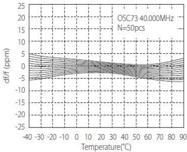
Frequency vs Temperature Characteristics
